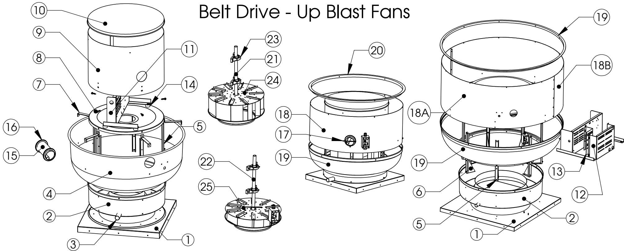
Belt Drive - Up Blast Fan - Part Information.
